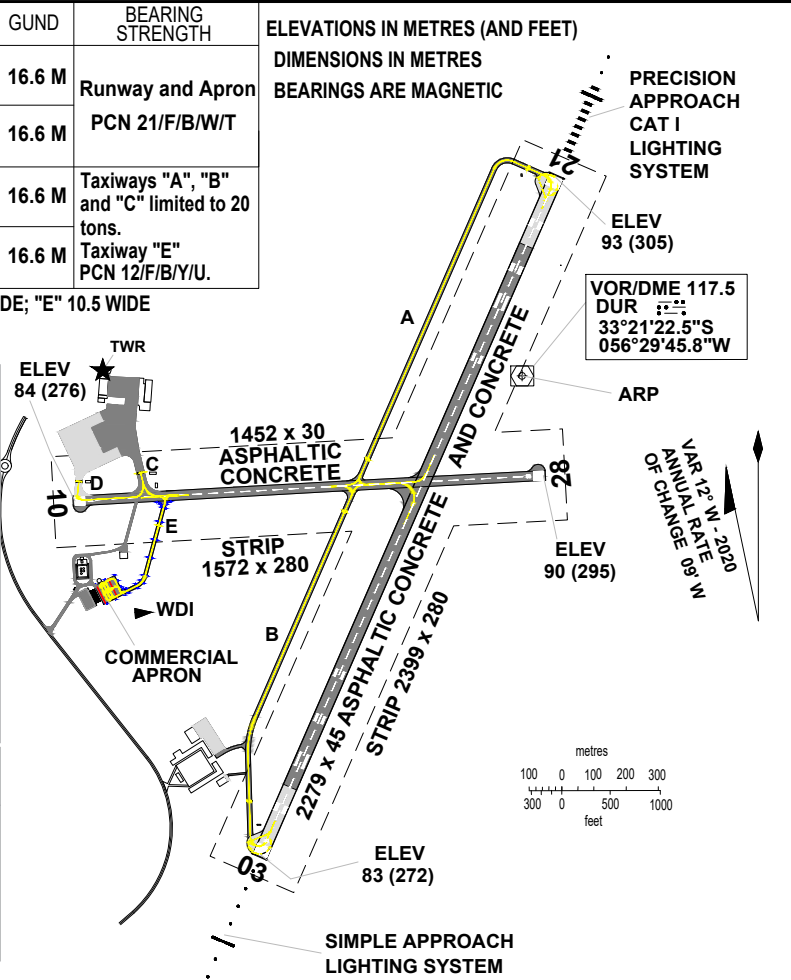
MARKING AIDS RWY 03/21 AND EXIT TWY
