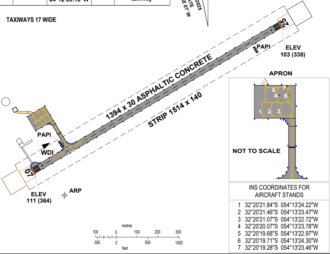
MARKING AIDS RWY 07/25 AND EXIT TWY
