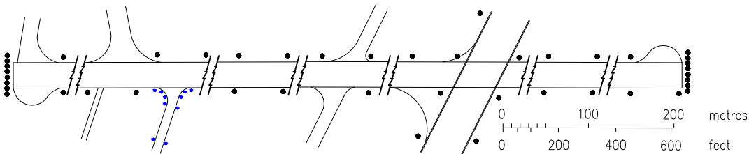
LIGHTING AIDS RWY 10/28 AND EXIT TWY
